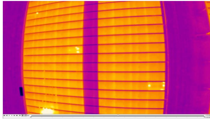
Figure 6: Infrared image of hot spots on solar panels in the OPTRIS software PI CONNECT
